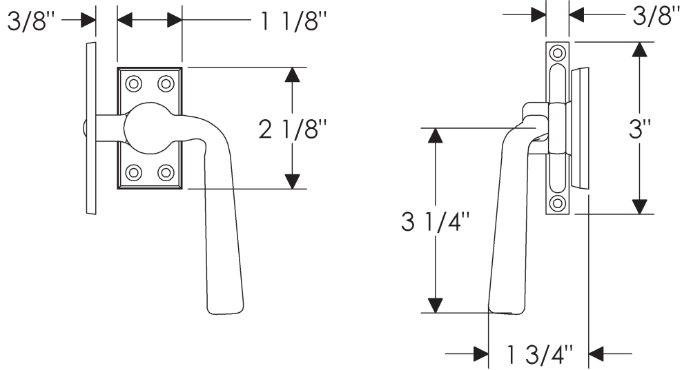
LC300 Casement Latch with LC303 Mortise Strike
