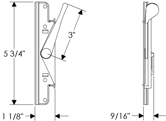
WL10 Sash Lock
