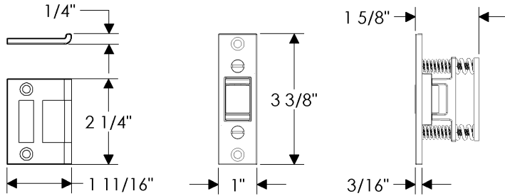
RL10 Roller Latch 1" x 3 3/8"
