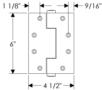
HNG6x4.5A Concealed Bearing Hinge 6"x 4.5"
