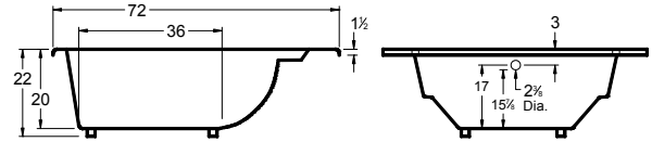
All bathtub dimensions are ± 1/2"
